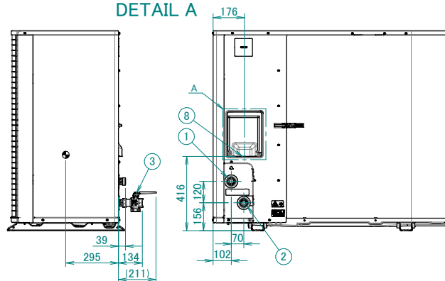
DETAIL A
